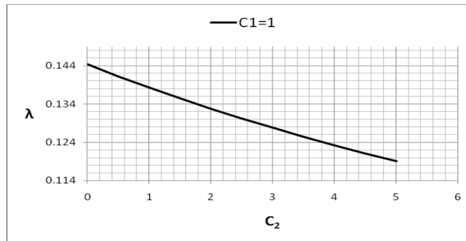
Fig. 3. Variation of \lambda versus C_2 for C_1 = 1
