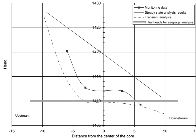
Fig. 18. Heads at instant 2 at elevation 1410 versus horizontal locations with respect to the center line of the core
