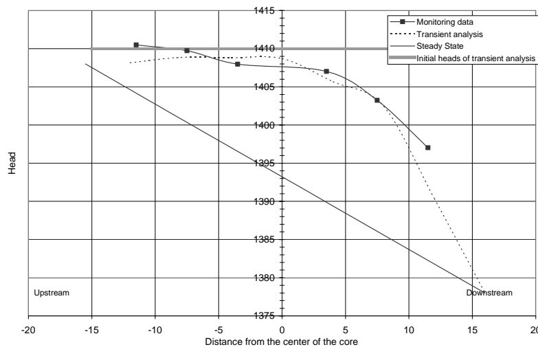
Fig. 12. Heads at instant 1 at elevation 1378 versus horizontal location with respect to the center line of the core
