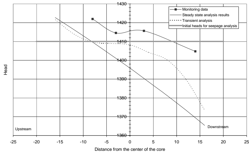
Fig. 15. Heads at instant 2 at elevation 1357.5 versus horizontal locations with respect to the center line of the core
