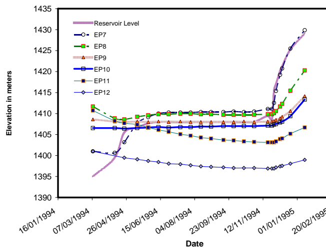
Fig. 5. Monitored heads in piezometers installed at elevation 1378
