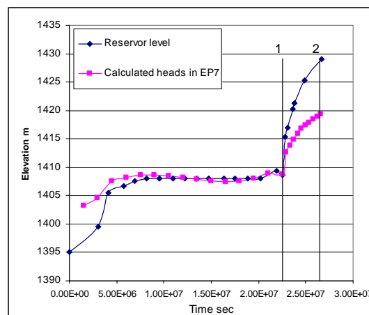
Fig. 10. Calculated heads in EP7 and reservoir level as functions of time
