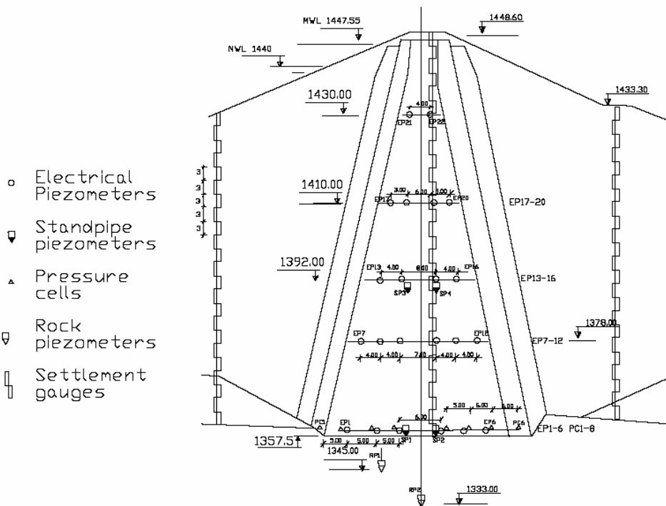
Fig. 2. Details of instrumentation at the monitoring section 3-3
