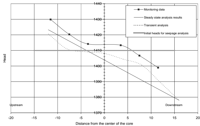
Fig. 16. Heads at instant 2 at elevation 1378 versus horizontal locations with respect to the center line of the core
