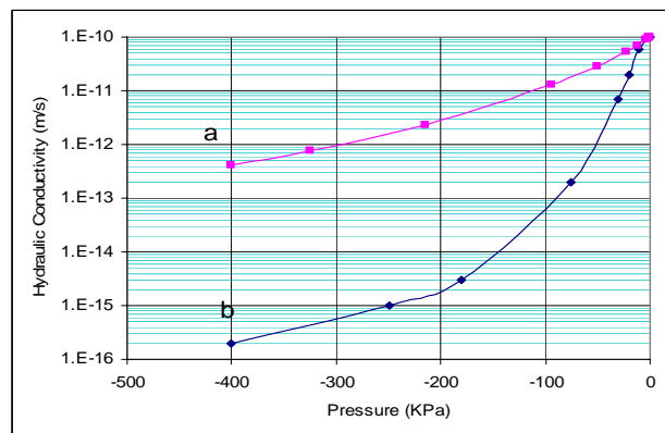
Fig. 8. Typical conductivity versus pressure functions used for unsaturated analyses of the core
