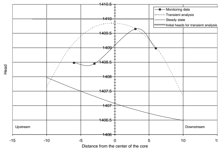
Fig. 14. Heads at instant 1 at elevation 1410 versus horizontal location with respect to the center line of the core
