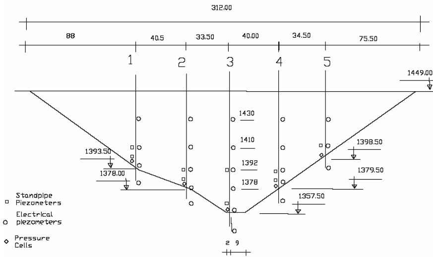
Fig. 1. Details of monitoring sections at the cross section of the dam valley
