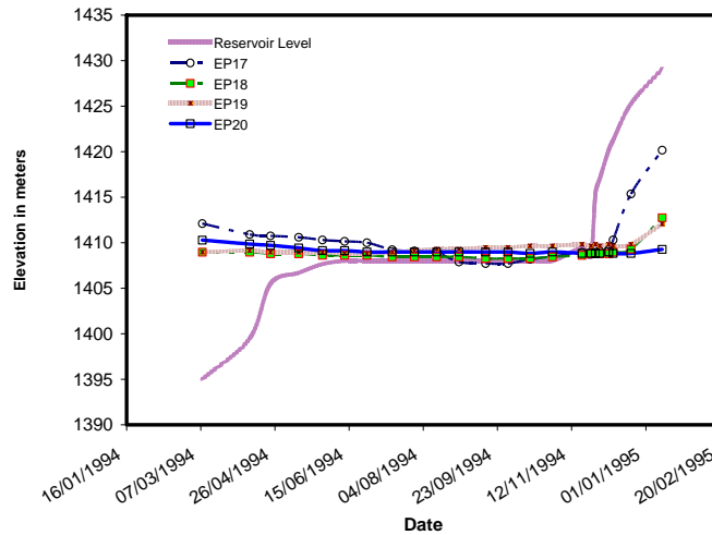
Fig. 7. Monitored heads in piezometers installed at elevation 1410
