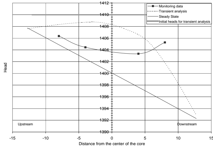
Fig. 13. Heads at instant 1 at elevation 1392 versus horizontal location with respect to the center line of the core
