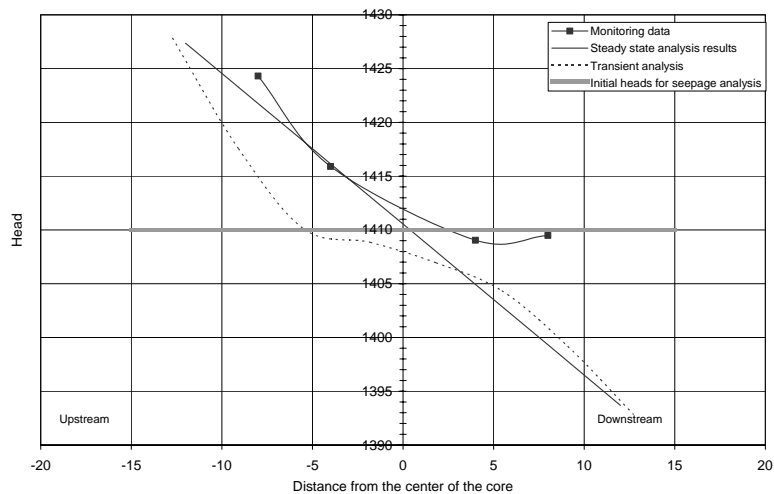
Fig. 17. Heads at instant 2 at elevation 1392 versus horizontal locations with respect to the center line of the core
