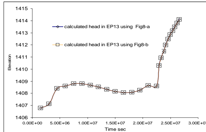
Fig. 9. Head versus time at EP13 obtained by application of two conductivity functions
