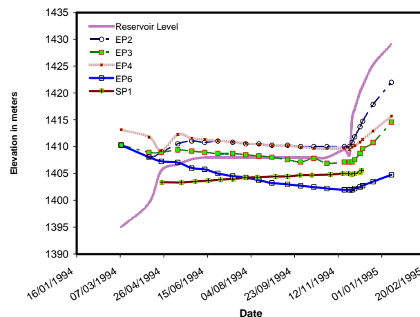
Fig. 4. Monitored heads in piezometers installed at elevation 1357.5
