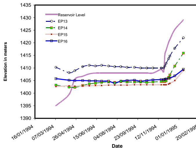
Fig. 6. Monitored heads in piezometers installed at elevation 1392
