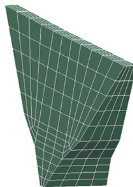
Fig. 3. Finite element mesh for the clayey core of 15-Khordad dam
