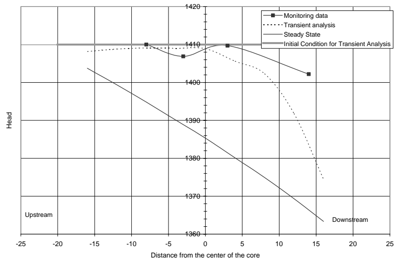
Fig. 11. Heads at instant 1 at elevation 1357.5 versus horizontal location
