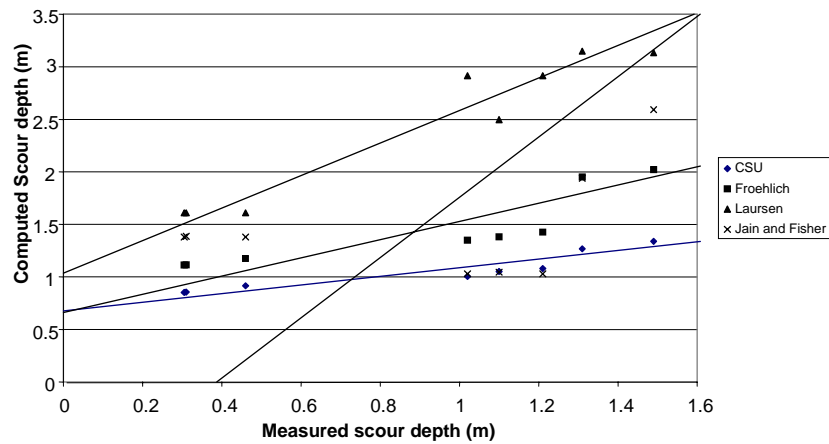
Fig. 2. Regression lines for fine materials for four equations
