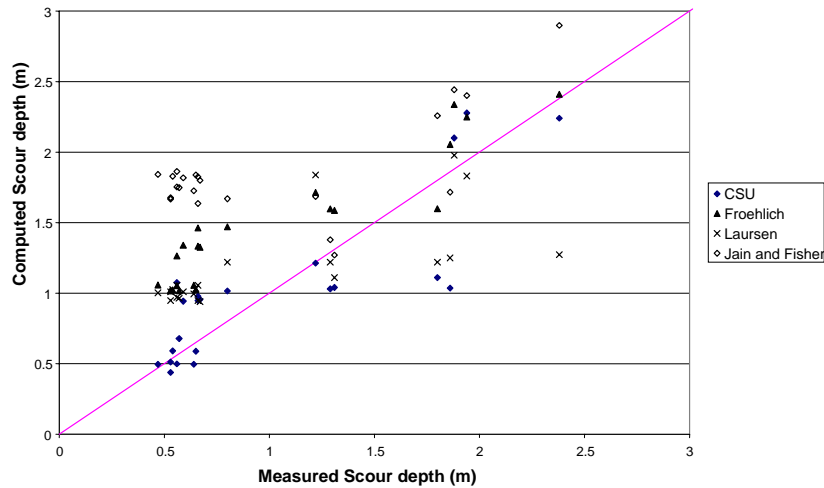
Fig. 7. Modified output by regression equation versus measured depth
